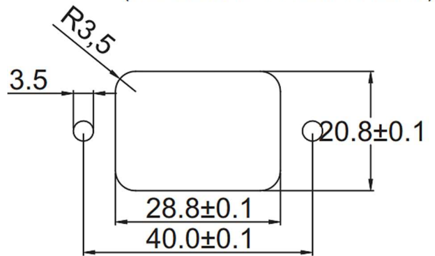
SUGGESTED PANEL CUTOUT (MOUNTING FROM FRONT)
